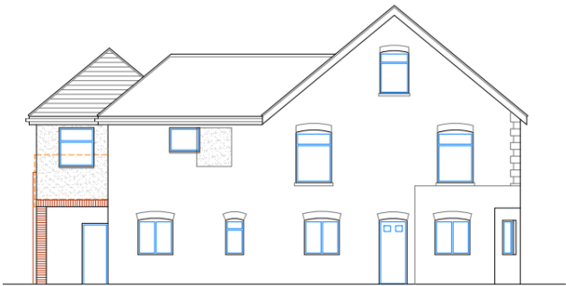
South Elevation
